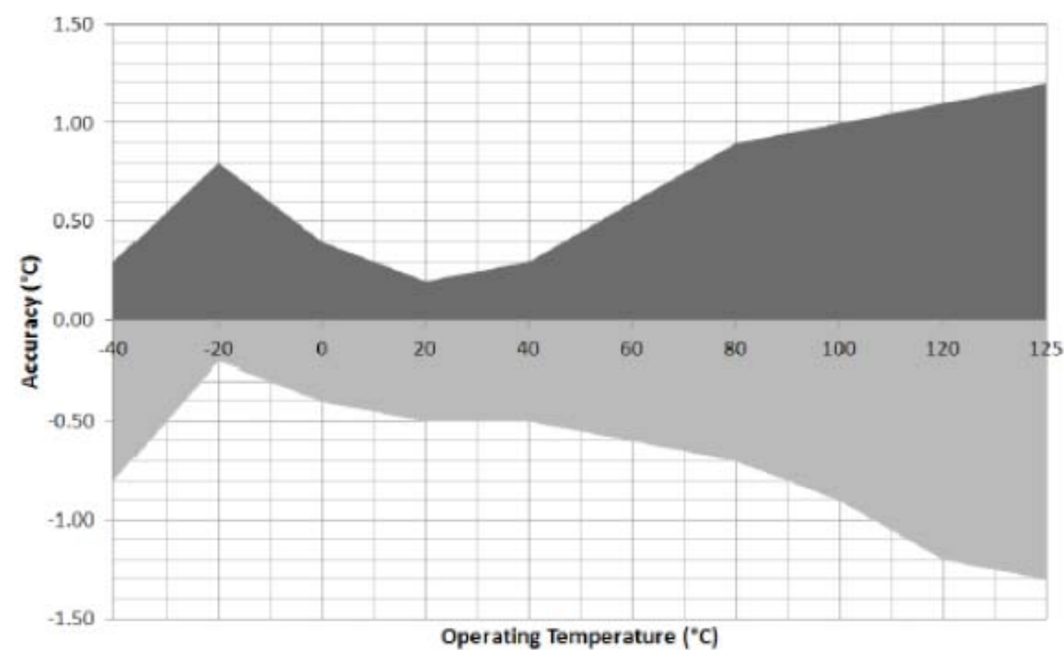
Supplied 'Type 2' Thermistor Probe Part Number: EL-PROBE2-1.0M-TP
