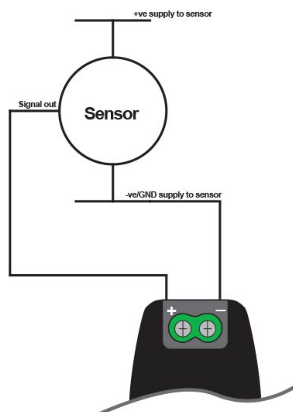
Logging a sensor voltage
